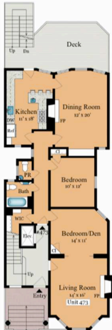
MAIN LEVEL
